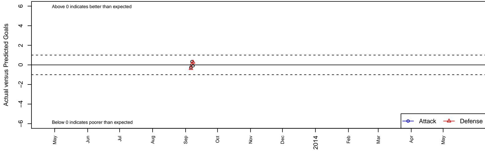
Spokane Foxes –Unk 2 G00 Dots are actual minus expected GF (blue circles) and GA (red triangles). Blue line is smoothed change in attack strength. Red is smoothed change in defense strength.
